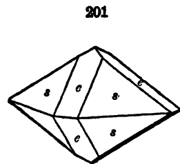
Cassiterite First and Second Order Pyramids
